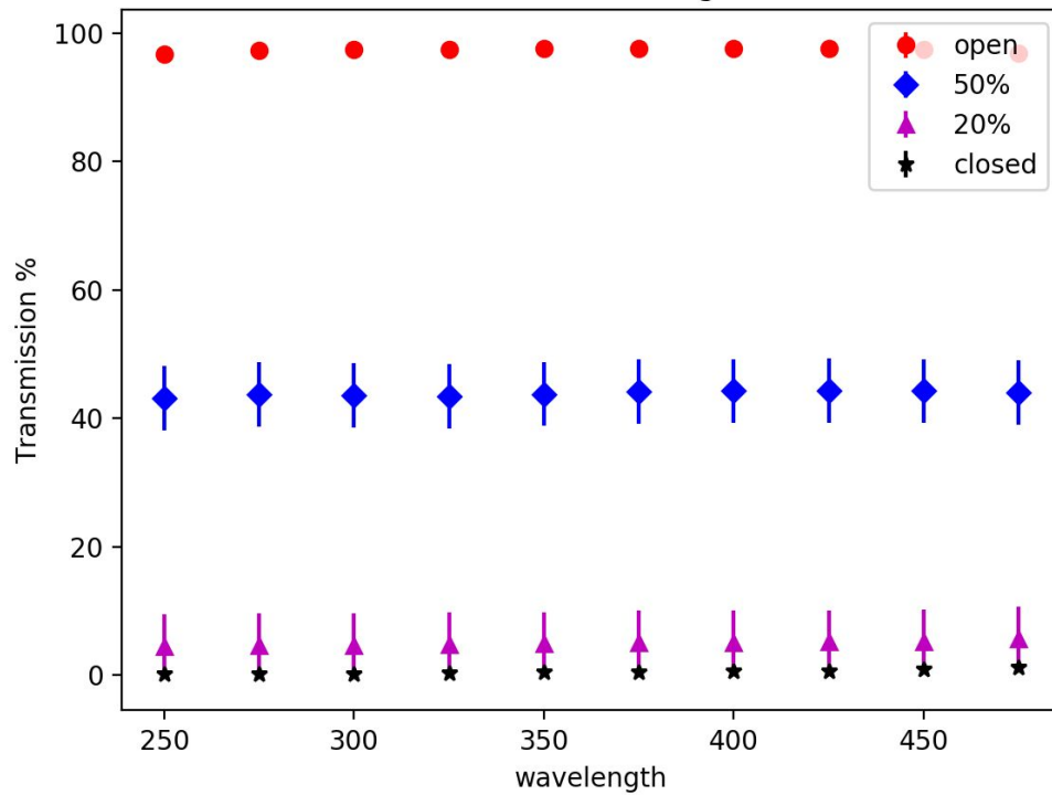
Transmission % using Irises
